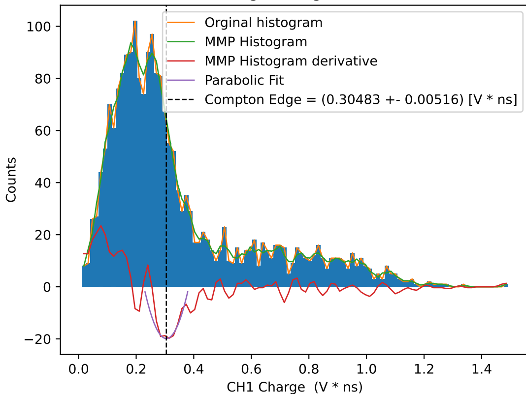
CH1 Charge histogram for 41V
